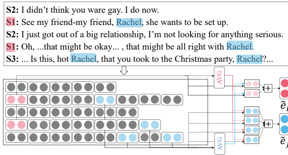
Figure 3: Mutual Attention for Entity Pair (Speaker1, Rachel)
